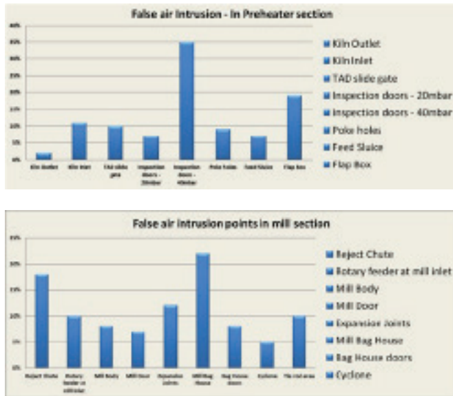
Fig. 01 False air intrusion points in Kiln & Mill section.
