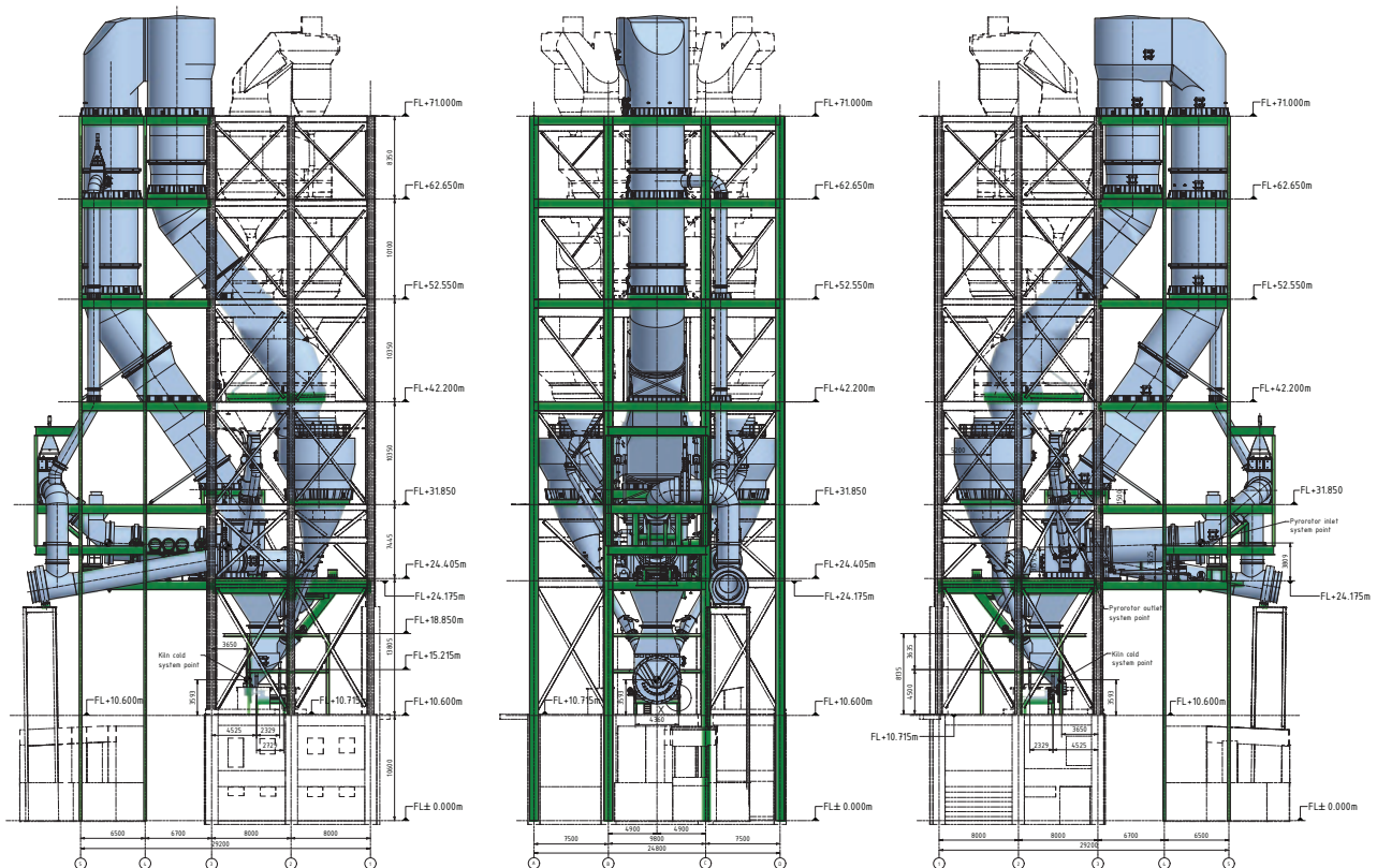
Figure 5: A Pyrorotor retrofit installation.
